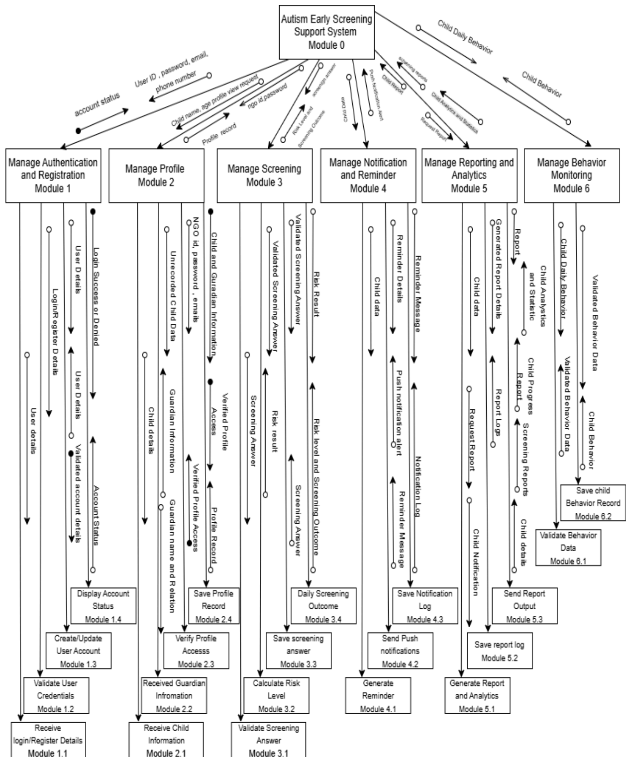
Diagram 28 : Structure Chart
