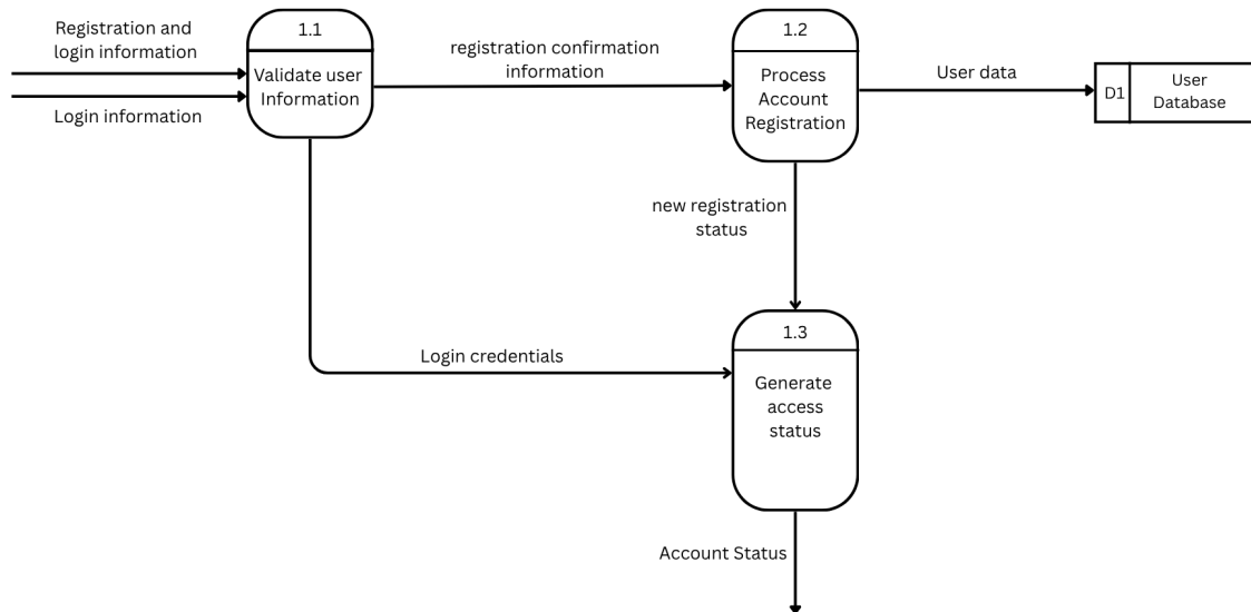
Diagram 9: Manage Authentication and Registration
