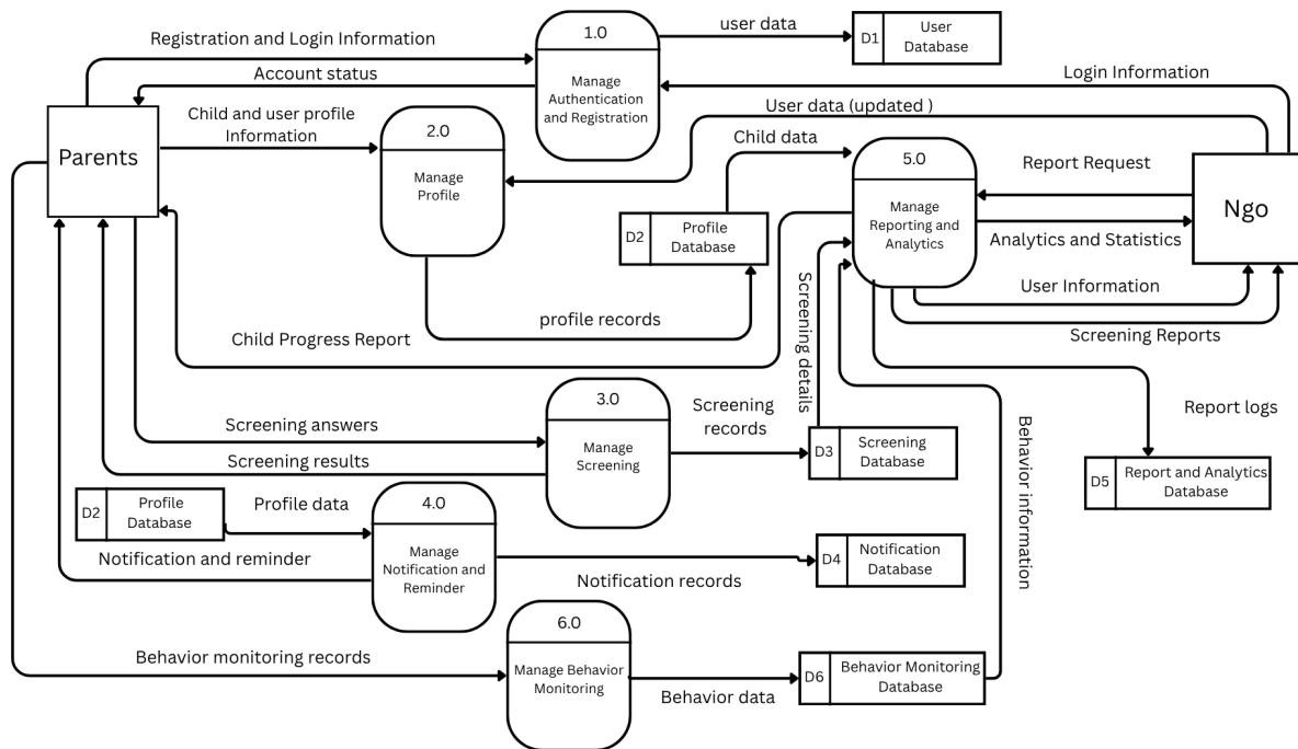
Diagram 8:Diagram 0 To-Be
