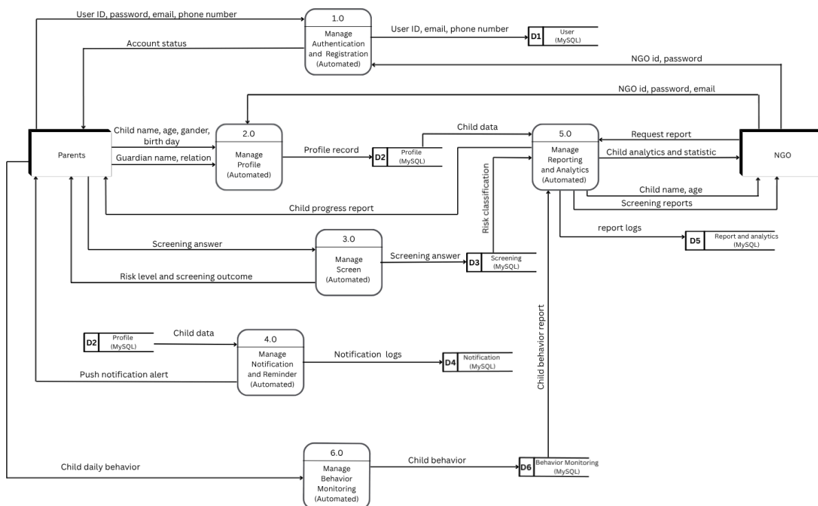
Diagram 14:Physical DFD TO-BE Diagram 0
