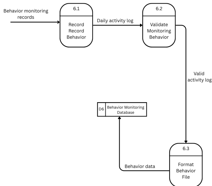
Diagram 14: Manage Behavior Monitoring
