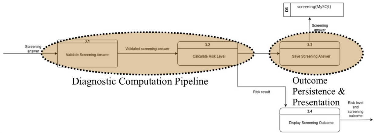
Diagram 24: Manage Screening
