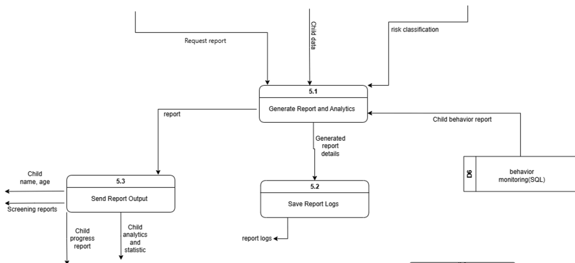
Diagram 19: Manage Reporting and Analytics
