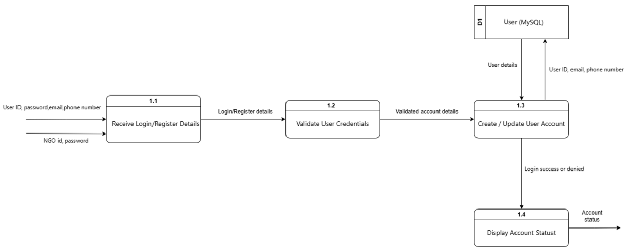
Diagram 15: Manage Authentication and Registration
