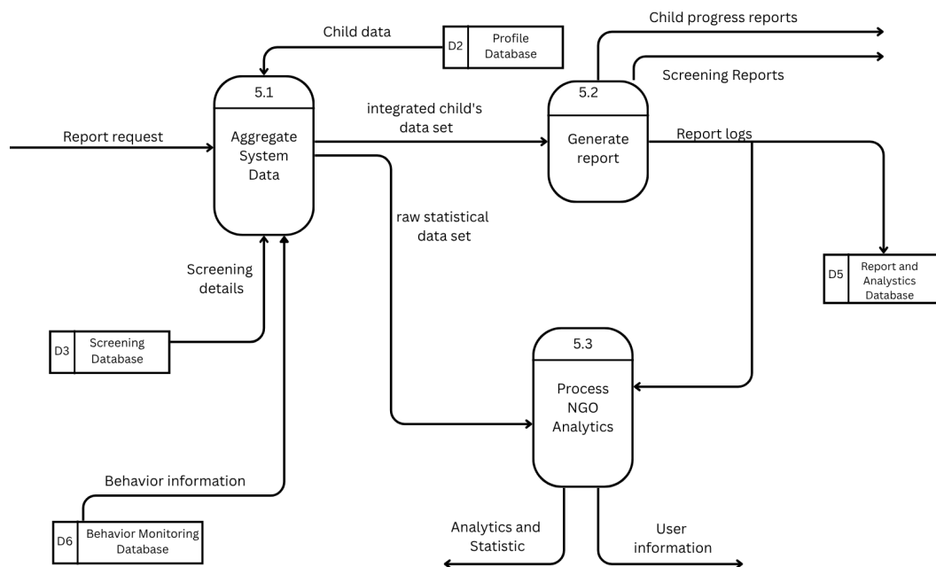
Diagram 13: Manage Reporting and Analytics
