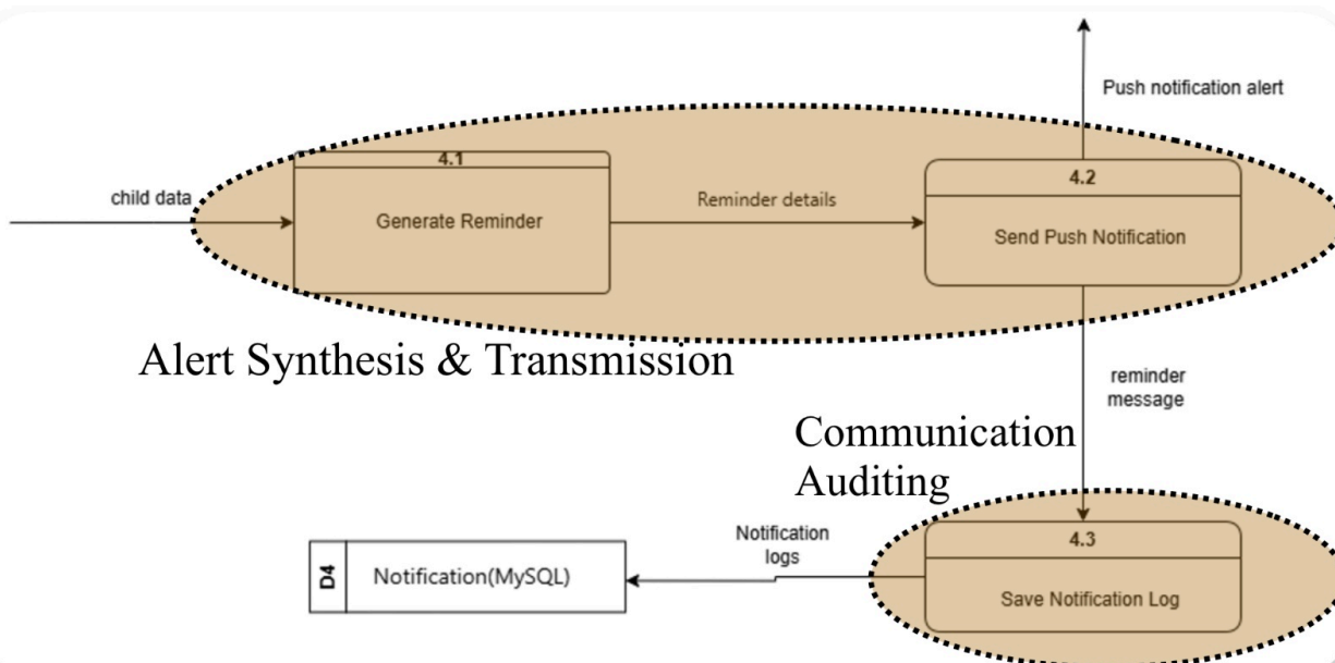
Diagram 25: Manage Notifications and Reminder
