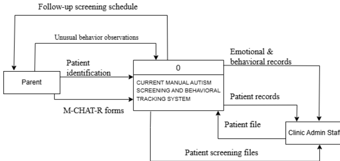
Diagram 2: Logical Context Diagram
