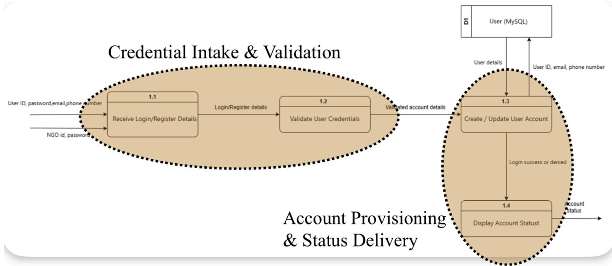
Diagram 22: Manage Authentication and Registration
