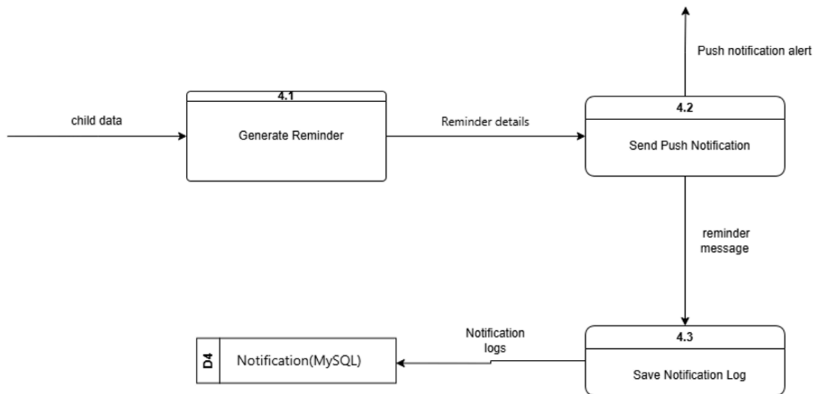
Diagram 18: Manage Notifications and Reminder
