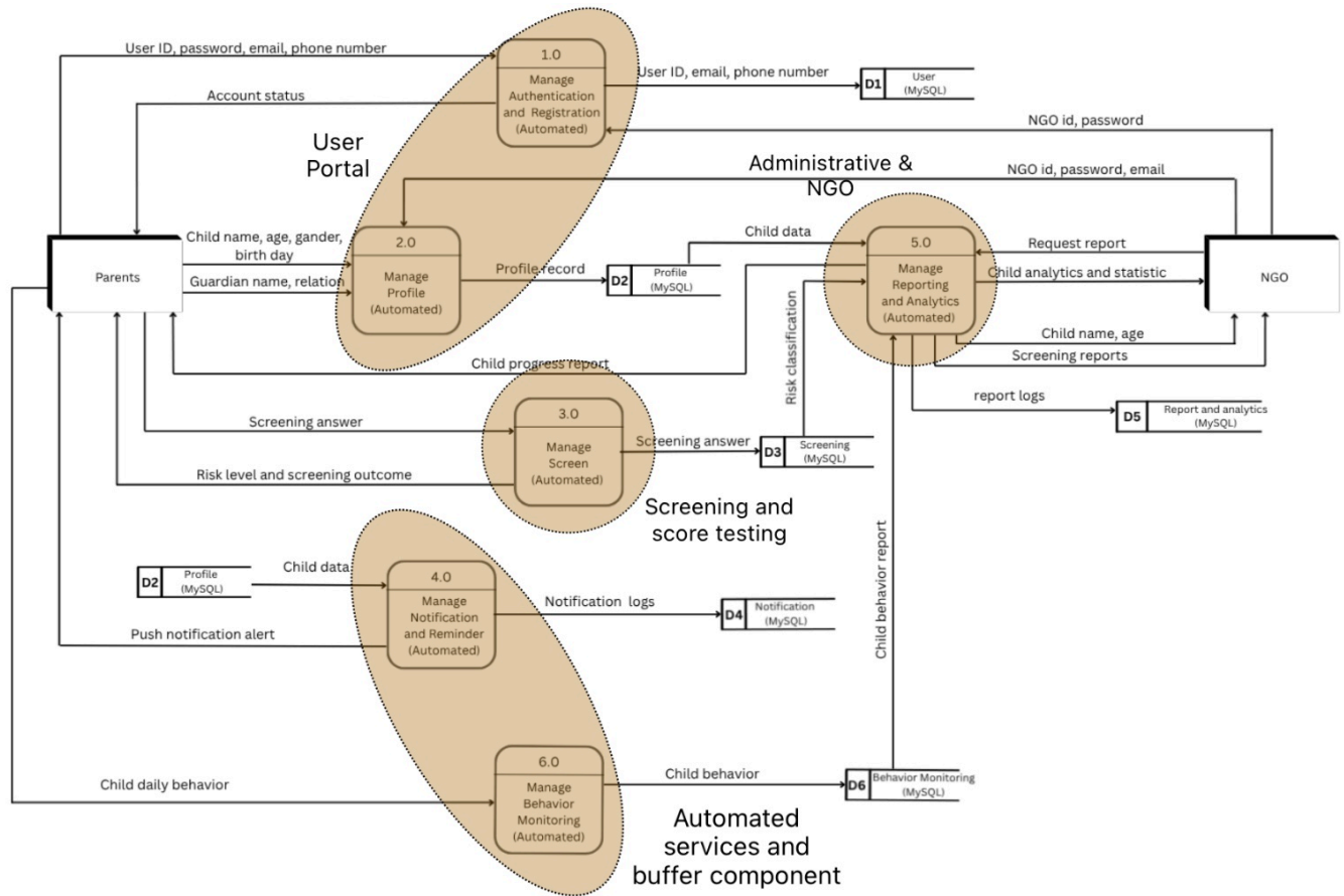
Diagram 21:Physical DFD TO-BE Partitioning
